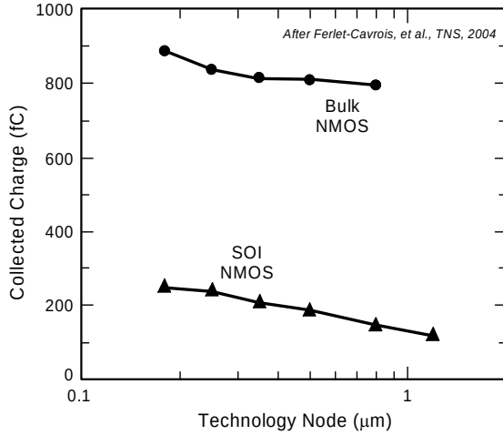
Fig. 9. Effect of scaling on charge collection predictions [18].
