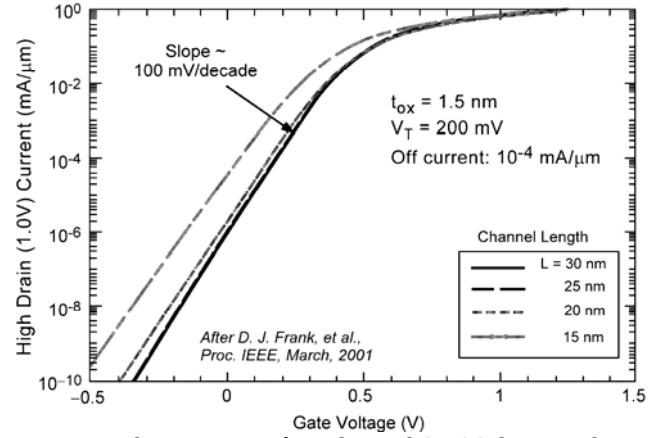
Fig. 5. I-V characteristics of an advanced CMOS device with channel lengths of 25 nm [9].
