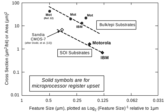
Fig. 14. Effect of scaling on saturation cross section for bulk and SOI microprocessors.
