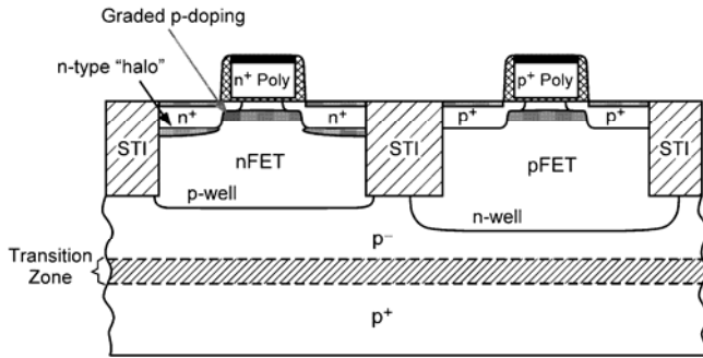
Fig. 4. Physical diagram of an advanced twin-well CMOS device on an epitaxial substrate.
