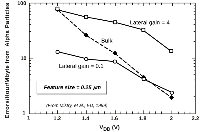
Figure 17 Effect of parasitic bipolar transistor gain on alpha-particle induced upset rates for SOI circuits [27].
