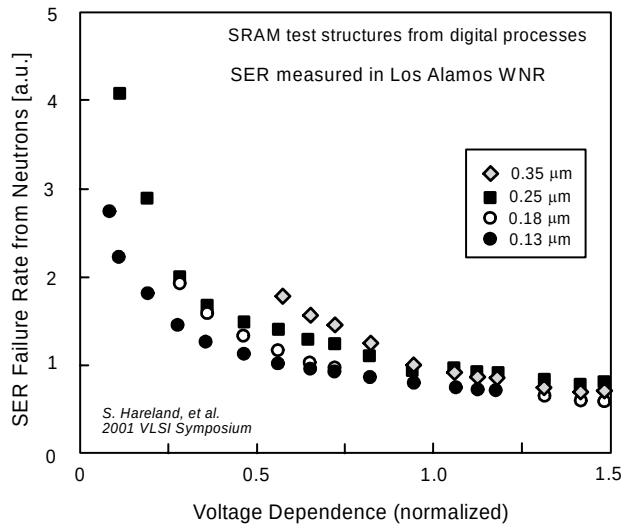
Fig. 19 Normalized neutron soft error rate for several technology generations, using SRAM test structures. Data were taken at the Los Alamos WNR facility.
