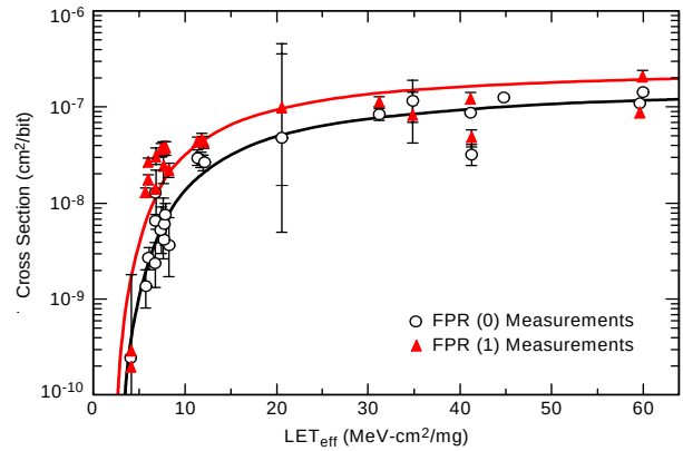
Figure 12. Upset cross section for floating-point registers in the Motorola Power PC750 microprocessor [21].
