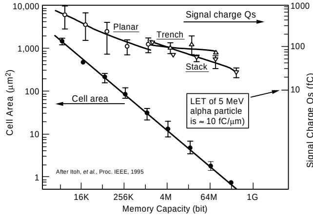
Fig. 3. Scaling predictions for DRAM technology.
