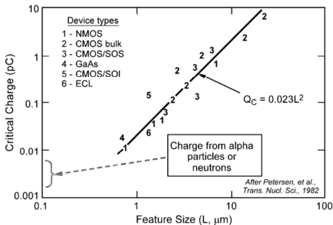
Fig. 1. Critical charge vs. feature size (after Petersen, et al. [2].) The figure has been revised to show the expected “plateau” from concern about alpha particles and atmospheric neutron effects.
