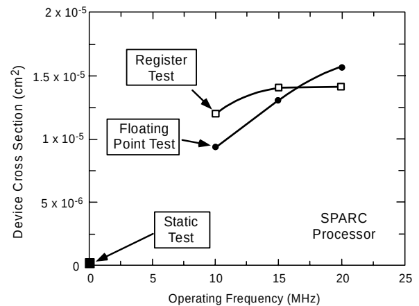
Fig. 15. Frequency dependence of upsets in an older SPARC processor.
