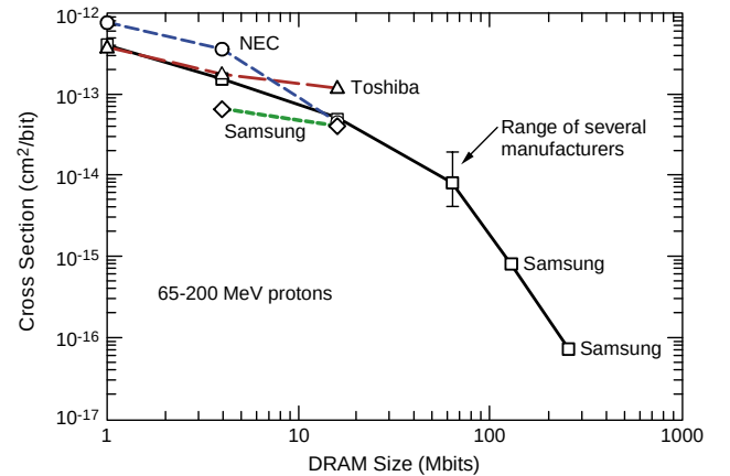
Fig. 10. Cross section for proton upset as DRAMs are scaled to smaller feature size.
