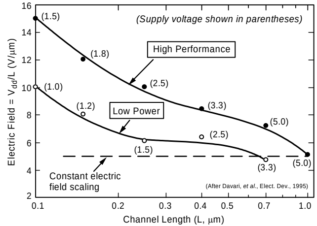
Fig. 2. Channel electric field and power supply voltage scaling predictions.
