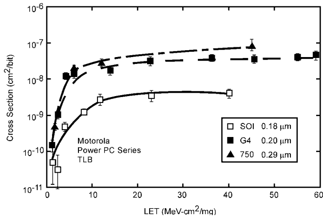
Figure 13. Register error rates for three generations of Power PC microprocessors from Motorola.
