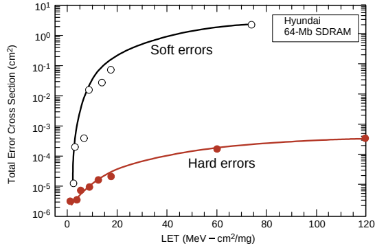
Figure 11. Upset and hard error cross section dependence on LET for an advanced DRAM.
