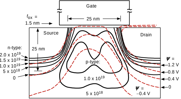
Fig. 6. Doping profile of an advanced NMOS transistor with gate length of 25 nm.
